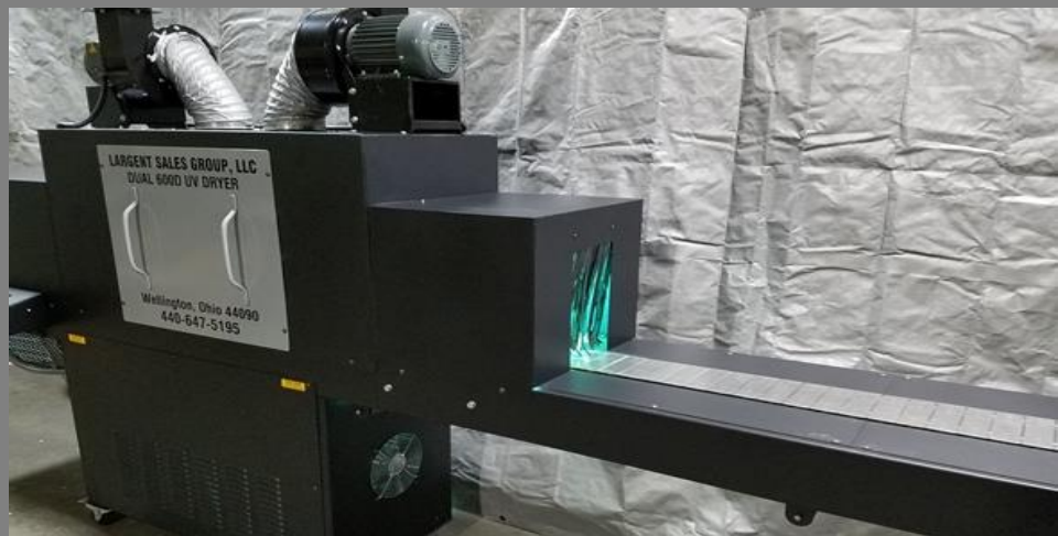
Metal-pallet conveying system for smooth continuous motion. Double chain with 4 corner drive system. Non-microwave system without microwave radiation. No radio frequency problems.
